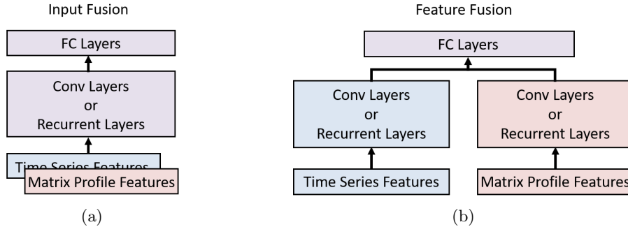
Fig. 2. Different arrangements of combining features in multi-modal fusion networks.
