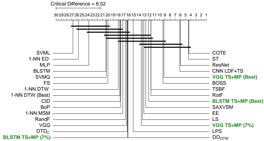
Fig. 3. Critical difference diagram using a Nemenyi test comparing the proposed method to reported methods. Green highlighted methods are the proposed input fusion networks.
