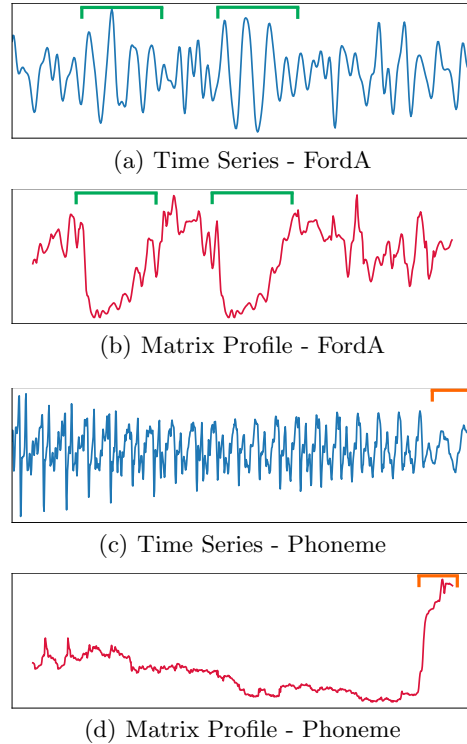
Fig. 1. Example of time series and the resulting Matrix Profile. The green brackets of (a) and (b) are an example of a motif, and the orange brackets of (c) and (d) are an example of a discord.
